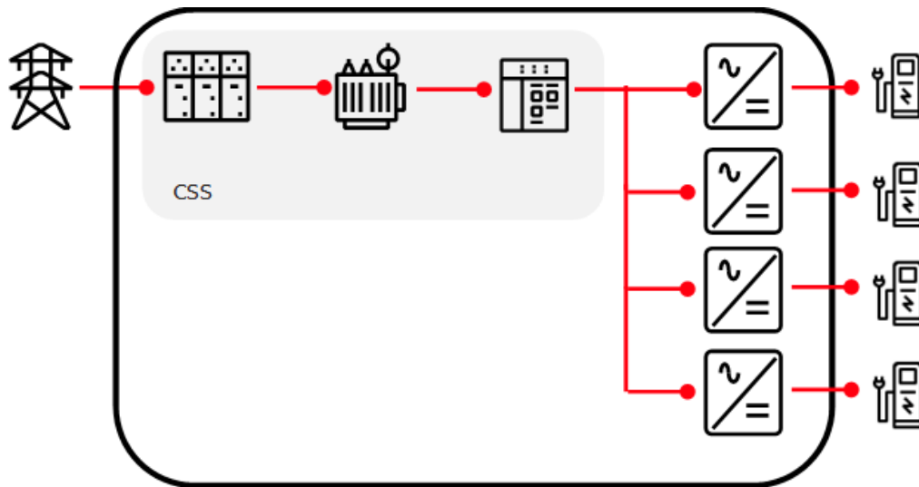
E-mobility skid-mounted CSS with integrated high-power chargers
