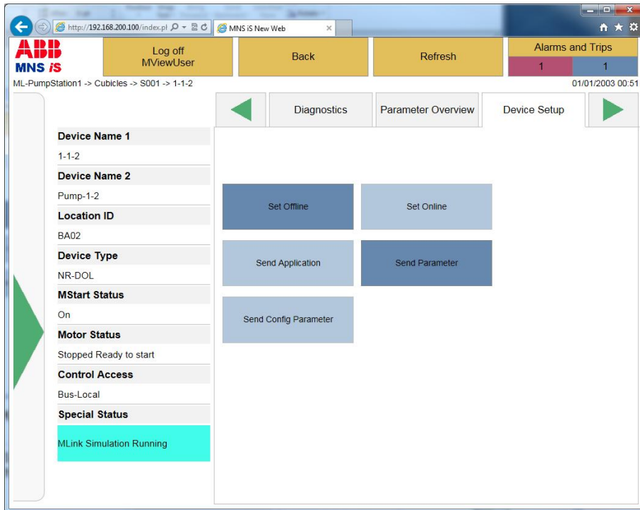
Figure 72 Device Details Page – MControl / MConnect – Device Setup
