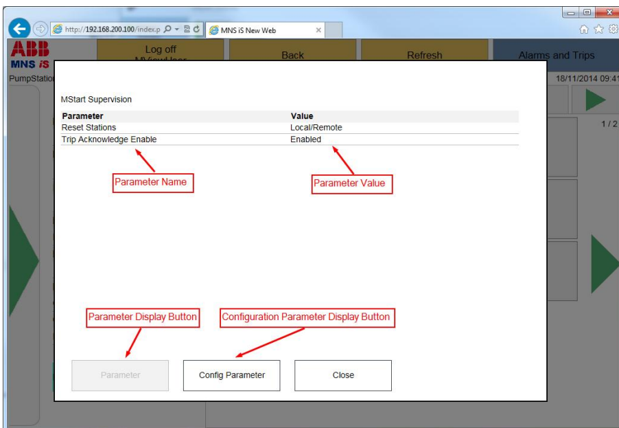
Figure 70 MControl parameter details
