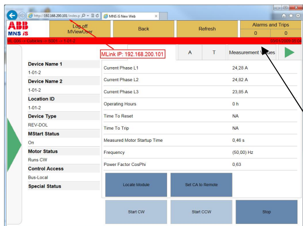
Figure 96 Screen after redundancy event
