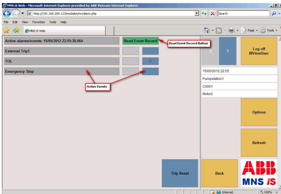
Figure 17 - Alarm view, current alarms
