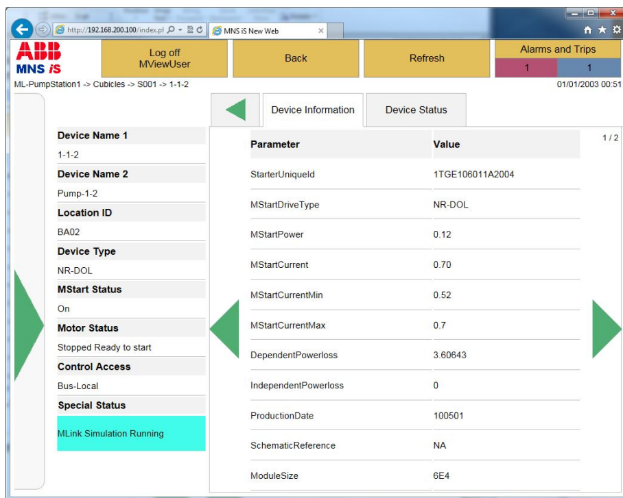
Figure 73 Device Details Page – MStart – Device Information
