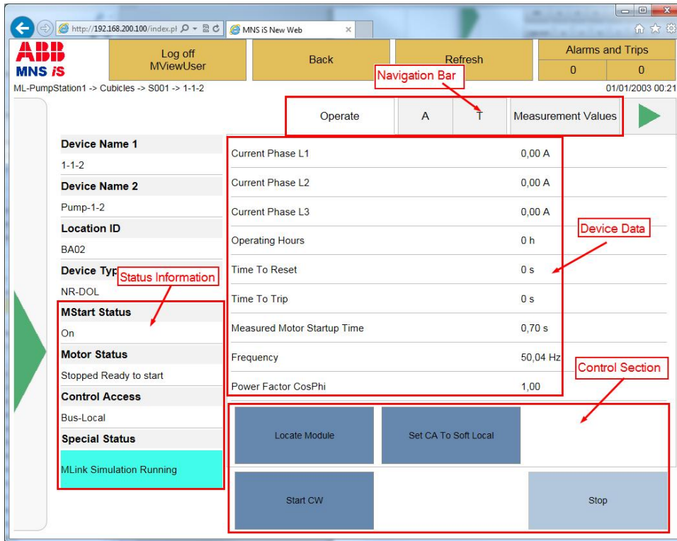
Figure 58 Device Details Page – MStart
