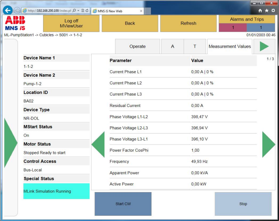
Figure 67 Device Details Page – MControl / MConnect - Measurement
