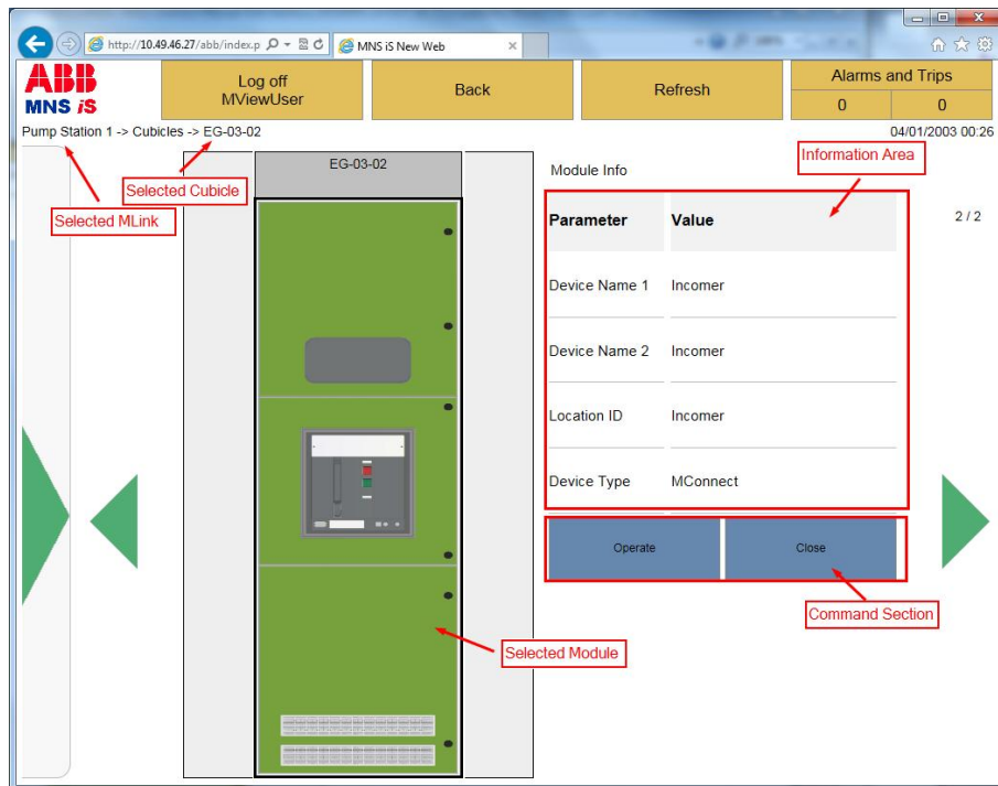
Figure 52 - Cubicle view* - Module (ACB + MConnect) selected
