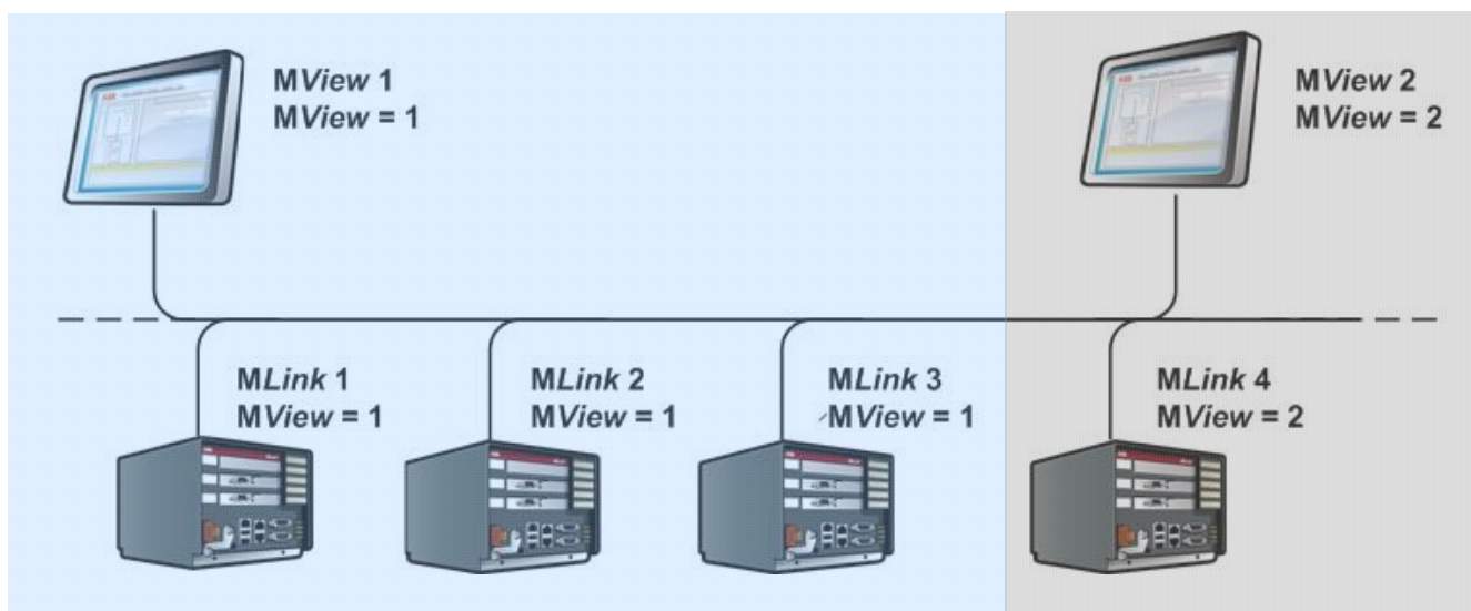
Figure 97 MView ID – Ethernet network segmentation
