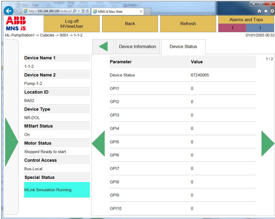
Figure 74 Device Details Page – MControl / MConnect – Device Status
