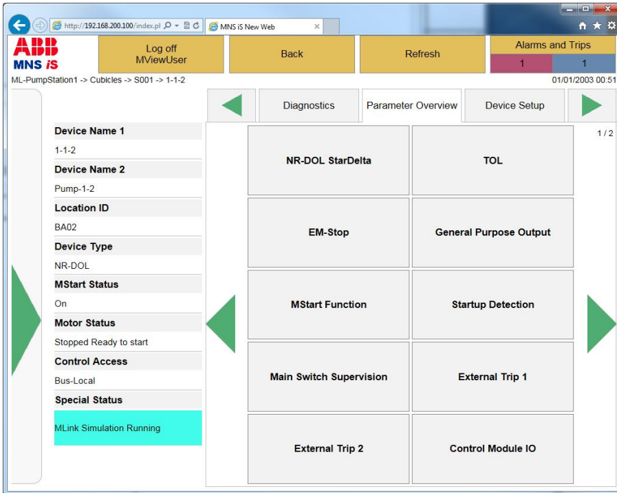
Figure 69 Device Details Page – MControl / MConnect – Parameter Overview
