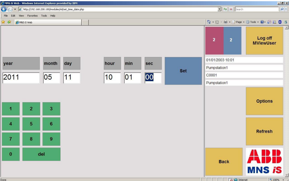
Figure 30 MLink Device Setup, setting RTC time
