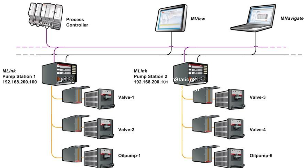
Figure 35 MNS iS System Structure
