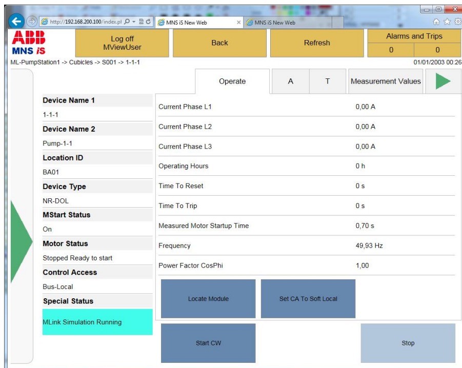
Figure 60 Device Details Page – MStart – Operate
