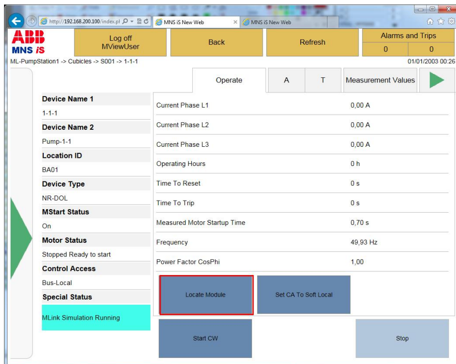
Figure 61: Locate Module Function in Operate Page
