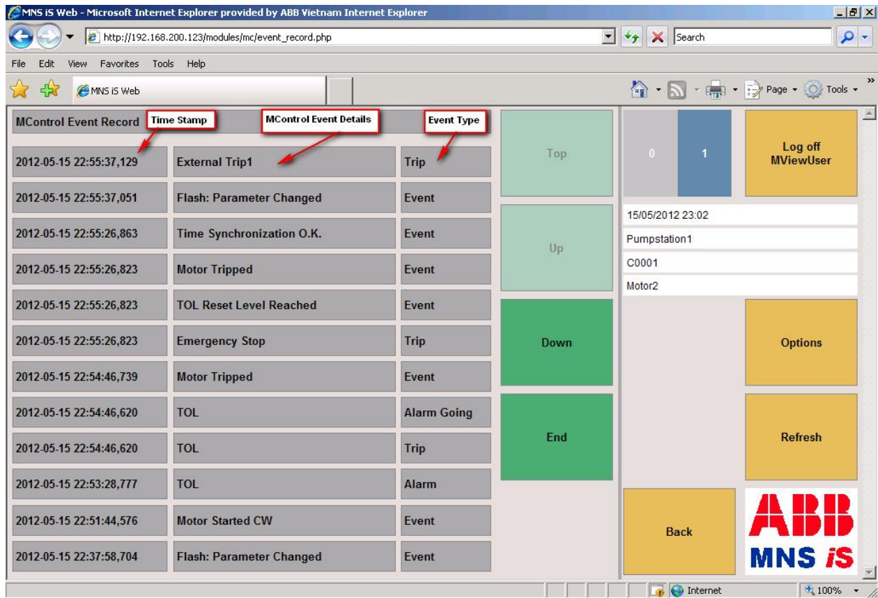
Figure 18 – Read Event Record
