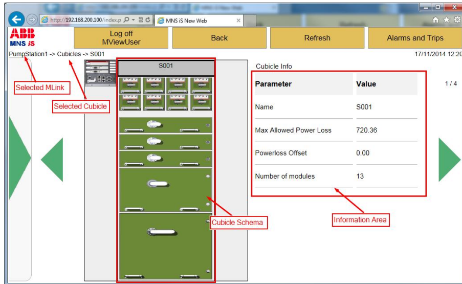
Figure 50 - Cubicle view* - Cubicle selected
