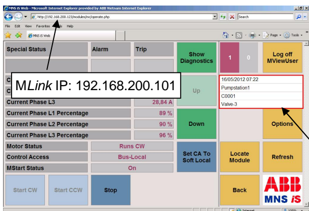
Figure 47 Screen after redundancy event
