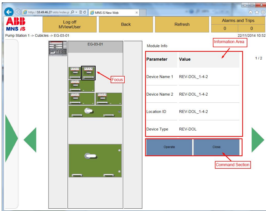
Figure 56 - Cubicle Navigation overview
