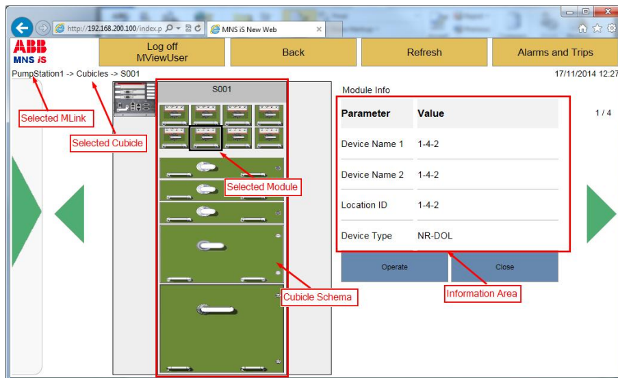
Figure 51 - Cubicle view* - Module ( MStart + MControl ) selected
