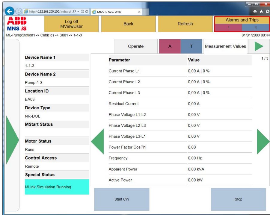
Figure 65: General Alarm/Trip Indication
