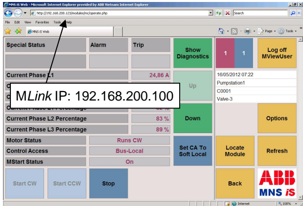
Figure 45 Screen before redundancy event
