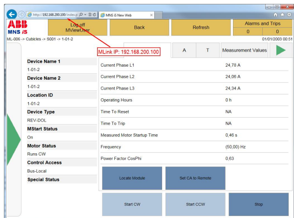
Figure 94 Screen before redundancy event
