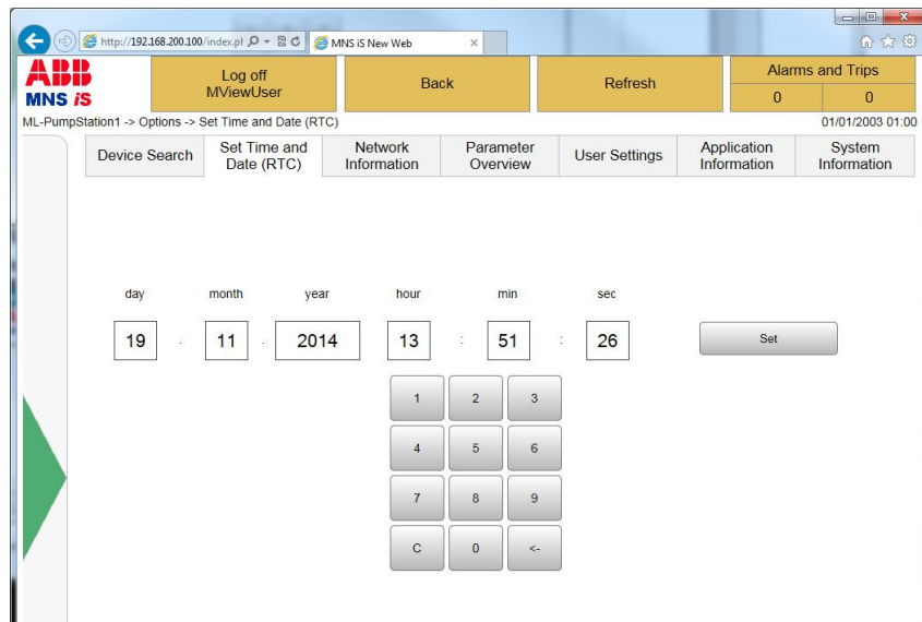
Figure 87 MLink Device Setup, RTC time synchronization
